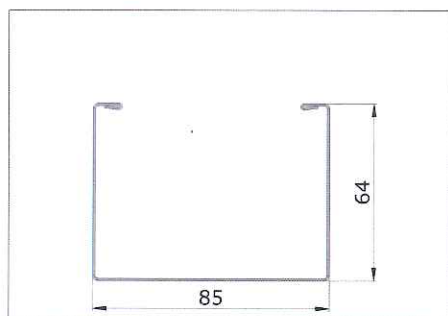
Ophang beugel
